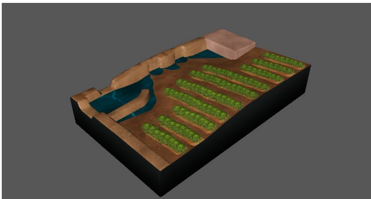
Figure 3.12: The SRP filled to the height of the emergency spillway. Along the headland cutouts can be seen dug into the bank. These further help to reduce the quantity of sediment that reaches the SRP. Consequently, reducing the accumulation of sediment in the pond which compromises the available storage and detention time, particularly in winter when the SRP cannot be cleaned out.
