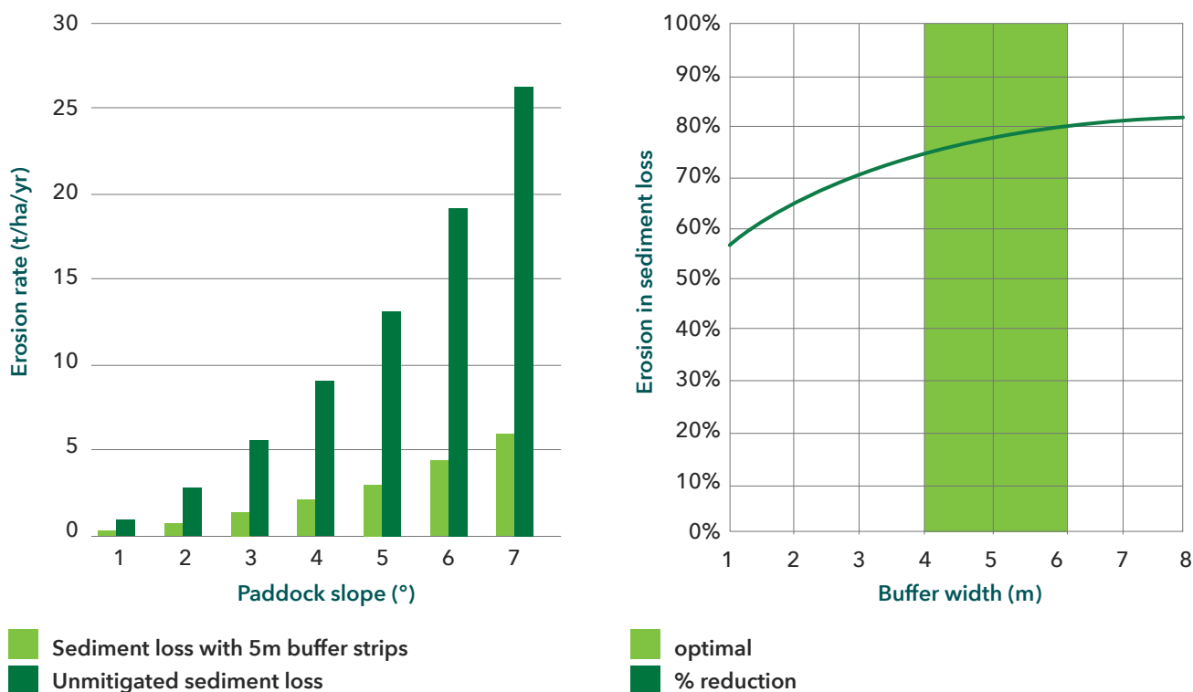
Figure 3.9: Modelled buffer strip efficiency based on paddock slope and buffer width (Location - Levin).
