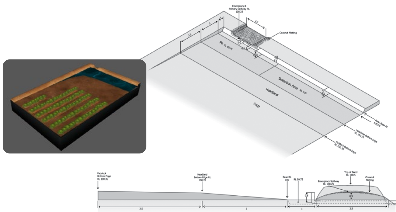
Figure 3.10: A 0.5m high decanting earth bund that uses the width of the block as its detention area. The headland was moved 4m further into the block.
